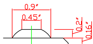
ENLARGED SECTION THROUGH DOME
